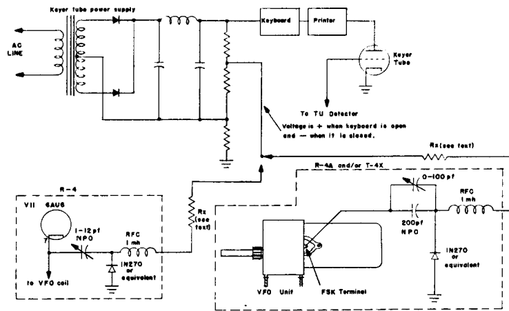
FIGURE 9 — FSK CIRCUITS
