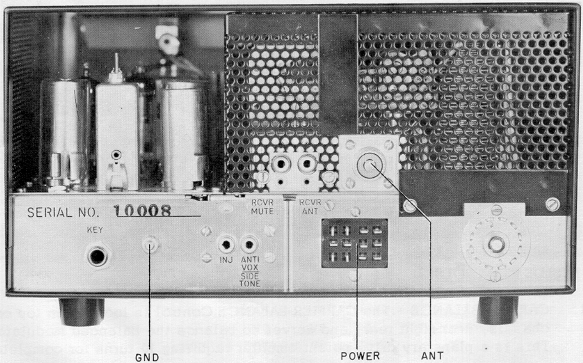
FIGURE 6 REAR VIEW
