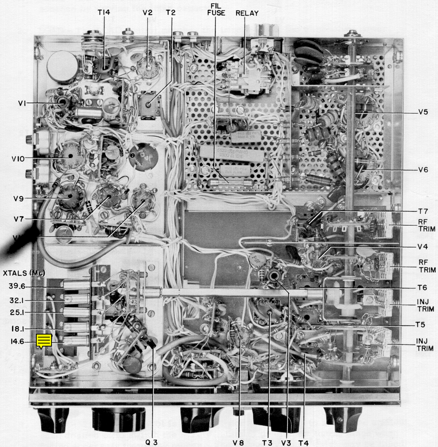
FIGURE 16 BOTTOM VIEW T-4X
