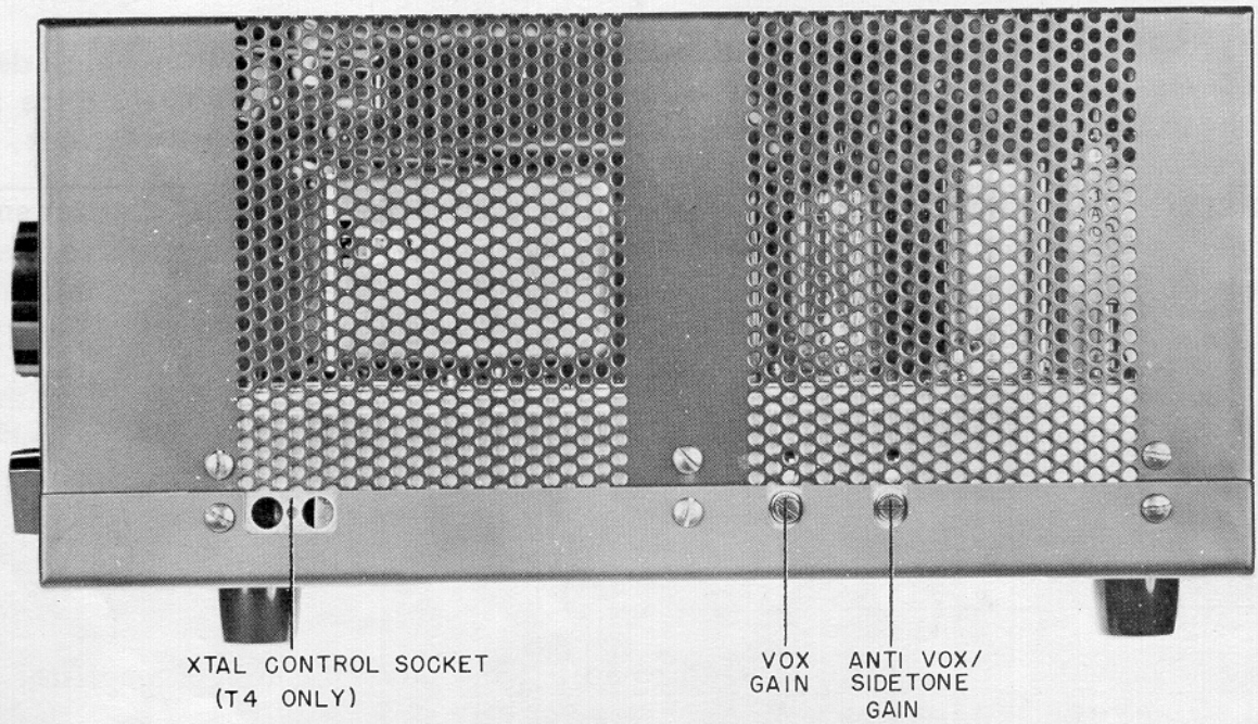
FIGURE 5 SIDE VIEW
